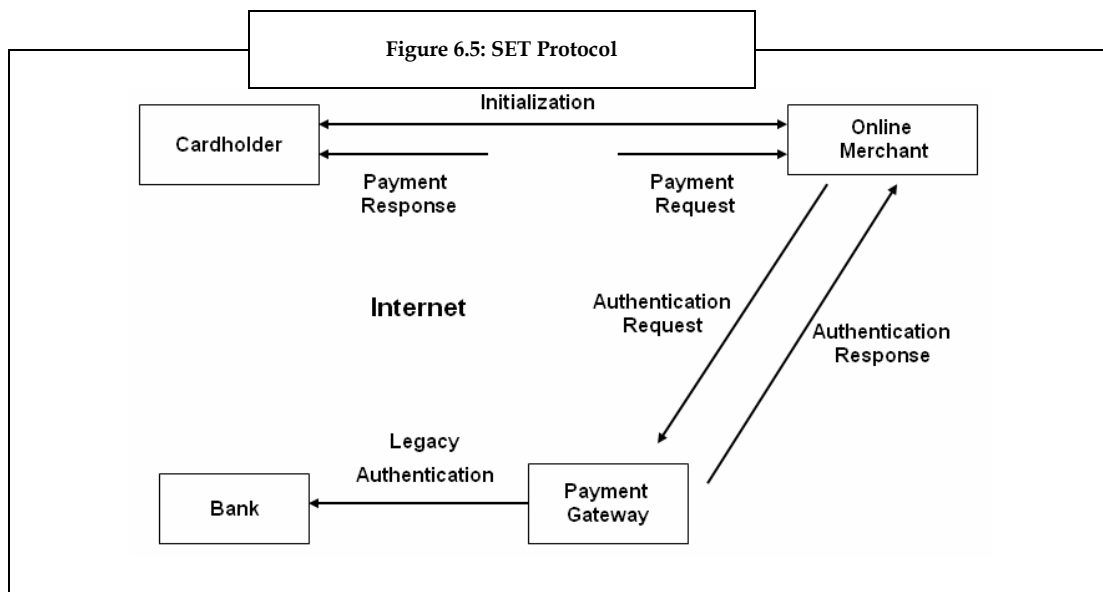
Figure 6.5 depicts SET Protocol.
